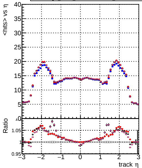
DOM mkFit Toriginal-106 DOM mkFit TNEWHSMS95 ALLITERS-106 DOM mkFit TNEWHSMS100 ALLITERS-106 mean hits
