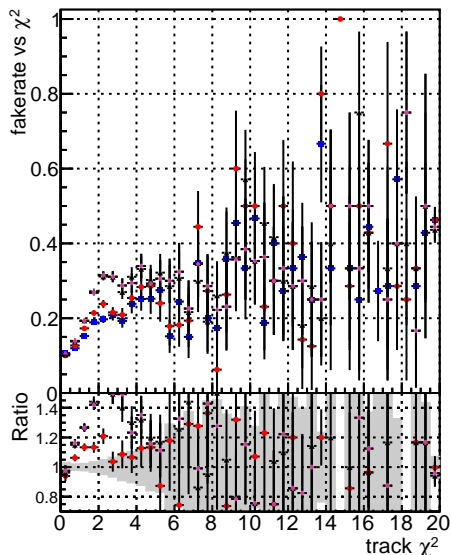
Fake rate vs. DOM mkFit TToriginal NEWHSM S100 ALLITERS-106 S100+ALLITERS-106
