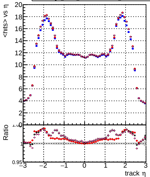
mean hits DOM mkFit Toriginal-106 DOM mkFit TNEWHSMS95 ALLITERS-106 DOM mkFit TNEWHSMS50 ALLITERS-106 DOM mkFit TNEWHSMS100 ALLITERS-106
