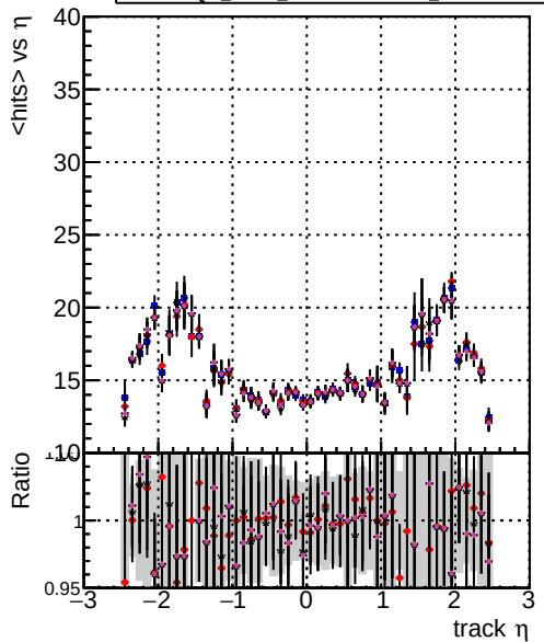
Legend: DQM mkFit Toriginal-106, DQM mkFit TNEWHSMS95 ALLITERS-106, DQM mkFit TNEWHSMS50 ALLITERS-106, DQM mkFit TNEWHSMS100 ALLITERS-106 mean hits
