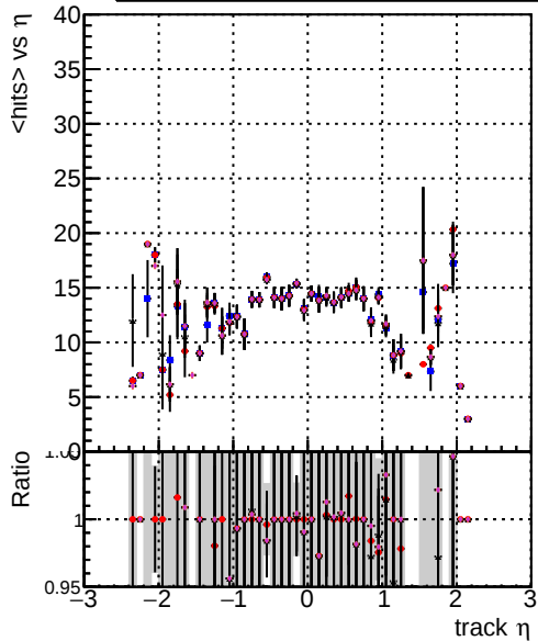
Legend: DQM mkFit Toriginal-106, DQM mkFit TNEWHSMS95 ALLITERS-106, DQM mkFit TNEWHSMS50 ALLITERS-106, DQM mkFit TNEWHSMS100 ALLITERS-106 mean hits
