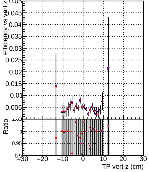
Efficiency vs. sim PV z Legend: - DOM mkFit TToriginal-106 - DOM mkFit TTNEWHSMS95 ALLITERS-106 - DOM mkFit TTNEWHSMS50 ALLITERS-106 - DOM mkFit TTNEWHSMS100 ALLITERS-106
