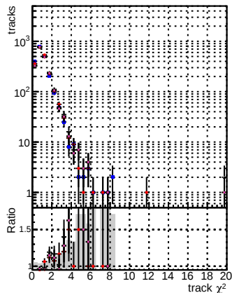
N of reco track vs. \chi^2 for different track types
