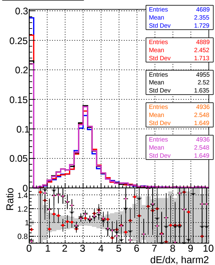
DOM_mkFit TToriginal DOM_mkFit TToriginal-106 DOM_mkFit TTNEWHSMS95_ALLITERS-106 DOM_mkFit TTNEWHSMS50_ALLITERS-106 DOM_mkFit TTNEWHSMS100_ALLITERS-106
