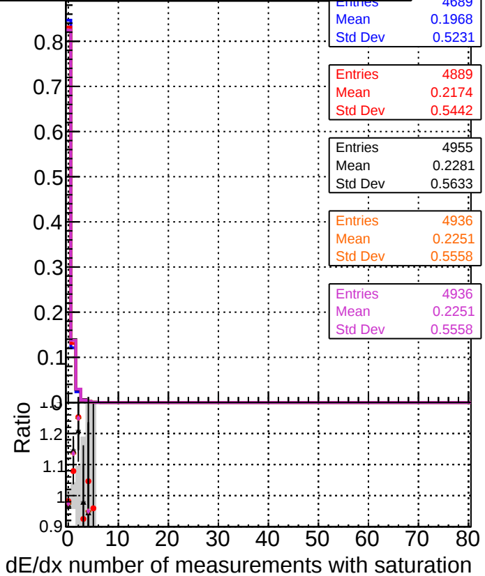
DOM_mkFit TToriginal DOM_mkFit TToriginal-106 DOM_mkFit TTNEWHSMS95_ALLITERS-106 DOM_mkFit TTNEWHSMS50_ALLITERS-106 DOM_mkFit TTNEWHSMS100_ALLITERS-106
