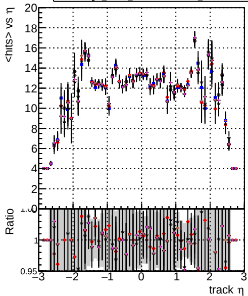
mean hit DOM mkFit Toriginal-106 DOM mkFit TNEWHSMS95 ALLITERS-106 DOM mkFit TNEWHSMS100 ALLITERS-106 DOM mkFit TNEWHSMS100 ALLITERS-106
