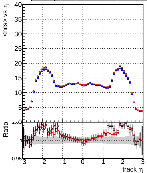
Legend for mean hits vs \eta : DOM mkFit TToriginal-106 DOM mkFit TTNEWHSMS95_ALLITERS-106 DOM mkFit TTNEWHSMS50_ALLITERS-106 DOM mkFit TTNEWHSMS100_ALLITERS-106
