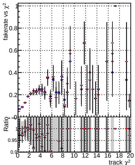
Fake rate vs. \chi^2 for DOM mkFit, TTERIGAL-105, TTERIGAL-106, NEWHSM3100, ALLTERS-106
