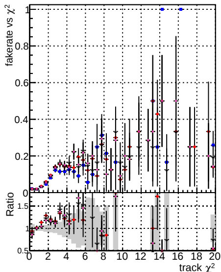
Fake rate vs. \chi^2 for various methods
