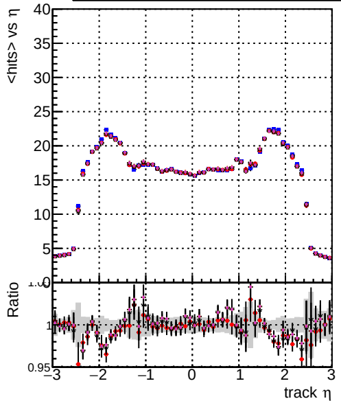
mean hit DOM mkFit TToriginal-106 DOM mkFit TTNEWHSMS95 ALLITERS-106 DOM mkFit TTNEWHSMS50 ALLITERS-106 DOM mkFit TTNEWHSMS100 ALLITERS-106
