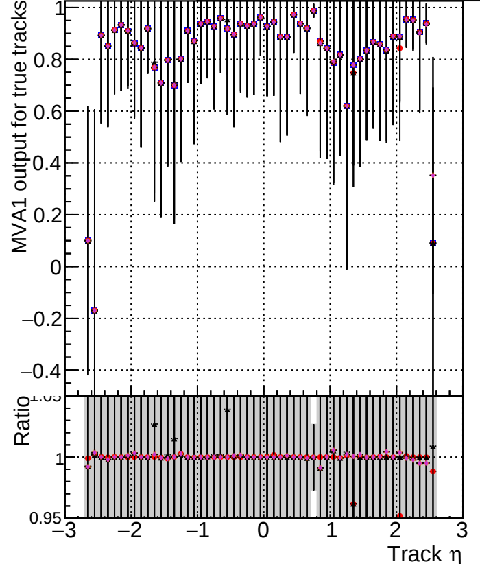
MVA1 of associated tracks (recoToSim) vs. track \eta Legend: DOM_mkFit_TToriginal DOM_mkFit_TToriginal-106 DOM_mkFit_TTNEWHSMS95_ALLITERS-106 DOM_mkFit_TTNEWHSMS50_ALLITERS-106 DOM_mkFit_TTNEWHSMS100_ALLITERS-106
