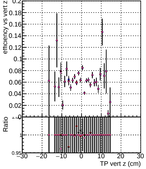
Efficiency vs. sim PV z — DOM mkFit TToriginal -106 — DOM mkFit TTNEWHSMS95 ALLITERS-106 — DOM mkFit TTNEWHSMS50 ALLITERS-106 — DOM mkFit TTNEWHSMS100 ALLITERS-106
