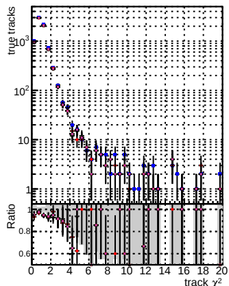
N of reco track vs. \chi^2 for different filter settings
