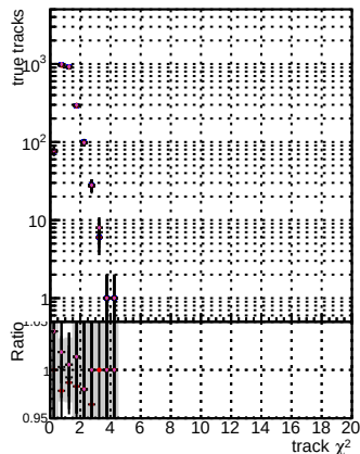
N of reco track vs. \chi^2 for different models and datasets
