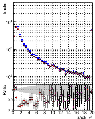
N of reco track vs. \chi^2 for BGM, mFit, TFit, and TFit+TFC
