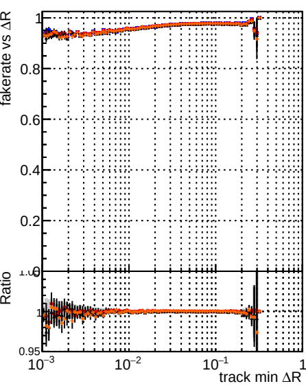
Fake rate vs \Delta R(\text{track, jet}) DOM mkFit Original-106 DOM mkFit NEWHSMS95 ALLTERS-106
