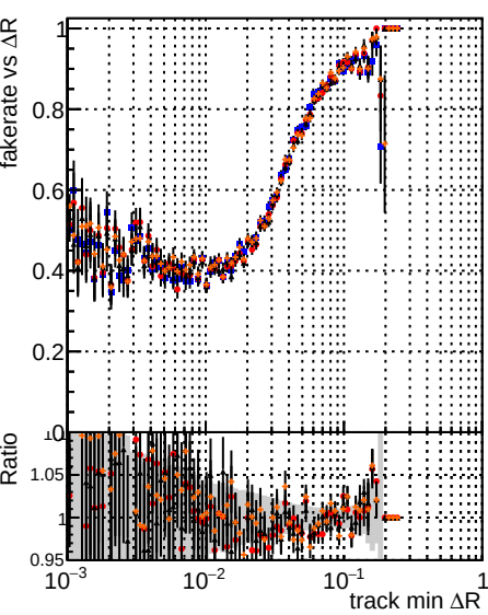
Fake rate vs \Delta R(\text{track, jet}) Legend: DOM (black), mkFit (blue), Toriginal (red), TNEW (orange) ALLITERS-106 NEWHSMS95 ORIGINAL-106
