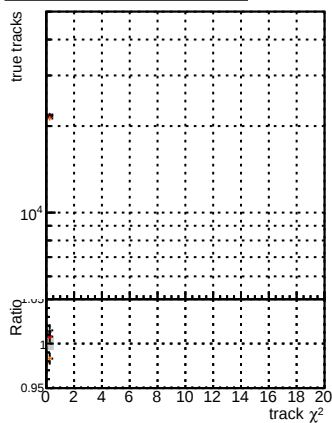
N of reco track vs. \chi^2 for BSM model: BSM model: T1000-100
