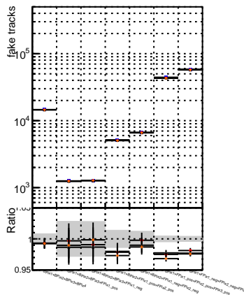
N of associated (recoToSim) fake tracks vs. \chi^2 for different track sets
