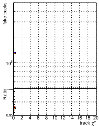
N of associated (recoToSim) fake tracks vs. \chi^2 for different track sets
