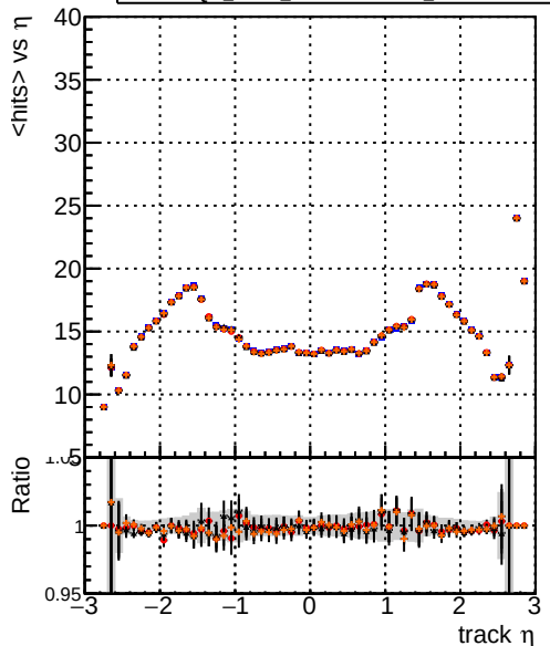
mean hits Legend: DQM_mkFit_TToriginal (blue line), DQM_mkFit_TToriginal-106 (red line with dots), DQM_mkFit_TTNEWHSMS95_ALLITERS-106 (black line with dots), DQM_mkFit_TTNEWHSMS90_ALLITERS-106 (orange line with dots)
