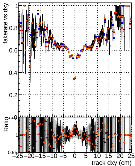
Legend: DGM mkFit (black), T-Original (blue), T-NEW (orange), T-ALLITERS (red)
