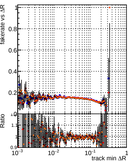
Fake rate vs \Delta R (track, jet) DOM mkFit Toriginal DOM mkFit Toriginal-106 DOM mkFit TNEWHSMS95 ALLITERS-106
