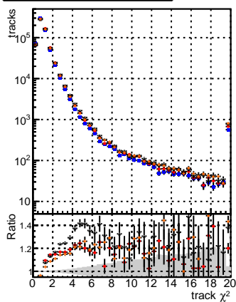
N of reco track vs. \chi^2 for BSM, mFit, Original, and NEWSM95 ALLITERS-106
