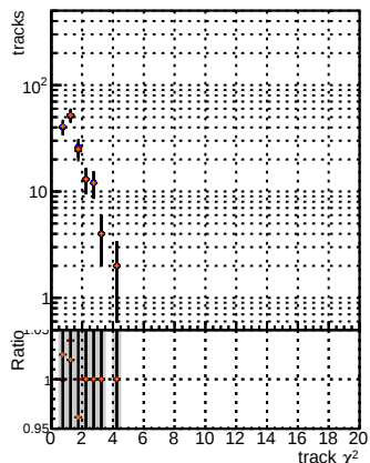
N of reco track vs. \chi^2 BSM mFit + Original vs BSM mFit + NEW vs ALLITERS-106
