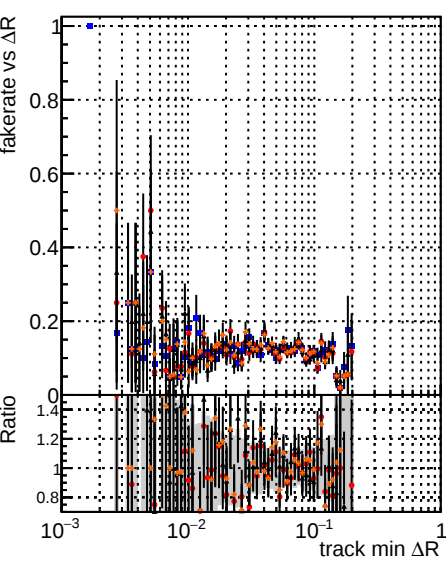
Fake rate vs \Delta R(\text{track, jet}) Legend: DOM (black), mktFit (blue), Toriginal (red), NEWHSMS95 (orange), ALLITERS-106 (green)
