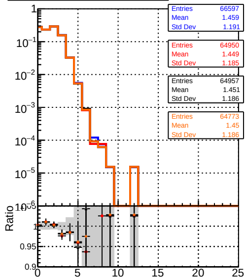
Legend: DQM_mkFit_TToriginal (blue line), DQM_mkFit_TToriginal-106 (red line), DQM_mkFit_TTNEWHSMS95_ALLITERS-106 (black line), DQM_mkFit_TTNEWHSMS90_ALLITERS-106 (orange line) mean hits
