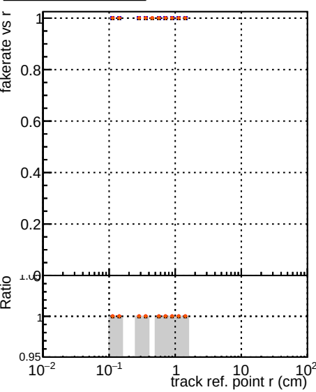
Fake rate vs v DOM mktFit Toriginal-106 DOM mktFit TNEWHSMS95 ALLITERS-106
