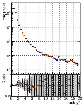
N of reco track vs. \chi^2 for BSM mFit, Original, BSM mFit, NEWMS-95, ALLITRS-106
