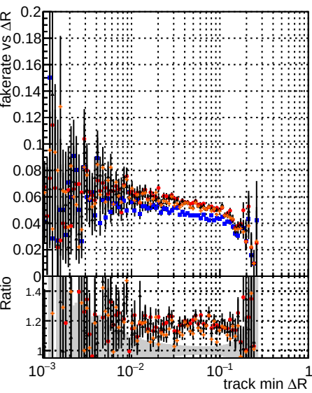
Fake rate vs \Delta R(\text{track, jet}) Legend: DOM mktFit Toriginal-106, DOM mktFit Toriginal-106, DOM mktFit TNEWHSMS95 ALLITERS-106
