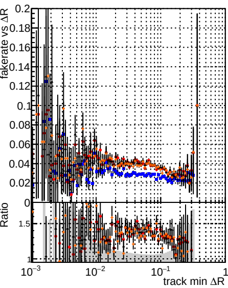
Fake rate vs \Delta R(\text{track, jet}) Legend: DOM mktFit T-Original T-What-106 DOM mktFit T-NEWHSMS95 ALLITERS-106
