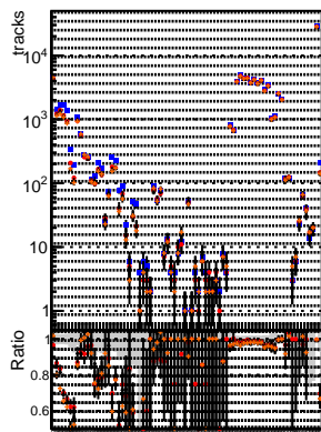
N of reco track vs. \chi^2 BGM mFit TFC original vs BGM mFit TFC NEWMS95 ALLITERS-106
