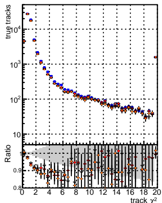
N of reco track vs. \chi^2 BGM mFit TFC original vs BGM mFit TFC NEWMS95 ALLITERS-106
