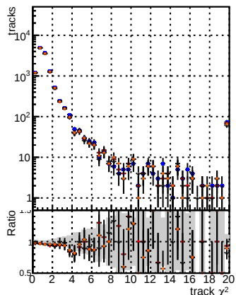
N of reco track vs. \chi^2 for BSM model TToriginal-05, BSM model TTNEWISM-95, and BSM model ALLITERS-106
