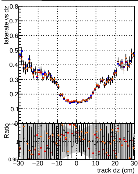
Fake rate vs dz Legend: DGM mkrFit (blue), T-Original (red), T-106 (orange), T-NEWHSM (black), ALLITERS-106 (grey), ALLITERS-95 (light grey).
