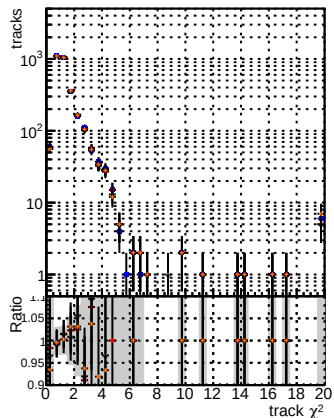
N of reco track vs. \chi^2 for BSM, mFEL, T1, T2, T3, T4, T5, T6, T7, T8, T9, T10, T11, T12, T13, T14, T15, T16, T17, T18, T19, T20, ALLITERS-106
