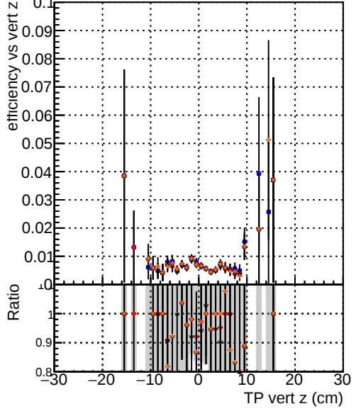
Efficiency vs. TP vert z —●— DQM_mkFit_TToriginal —●— DQM_mkFit_TToriginal-106 —●— DQM_mkFit_TTNEWHSMS95_ALLITERS-106 —●— DQM_mkFit_TTNEWHSMS90_ALLITERS-106
