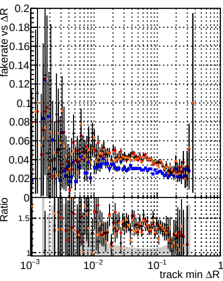
Fake rate vs \Delta R(\text{track, jet}) Legend: DOM (black), mktFit (blue), T-Original (red), T-What-106 (orange), NEWHSMS95 (grey), ALLITERS-106 (light grey).
