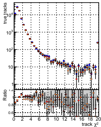
N of reco track vs. \chi^2 for BSM model TToriginal vs BSM model TTNEWHS95 ALLITERS-106
