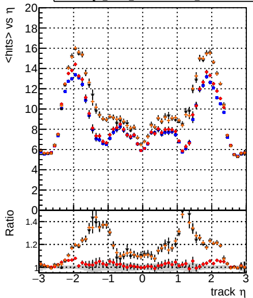
mean hit DQM_mkFit_TToriginal DQM_mkFit_TToriginal-106 DQM_mkFit_TTNEWHSMS95_ALLITERS-106 DQM_mkFit_TTNEWHSMS90_ALLITERS-106
