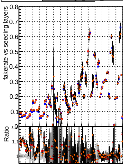
Fake rate vs. BQM mkFit T-Original 106 BQM mkFit T-NEWSMS95 ALLITERS-106
