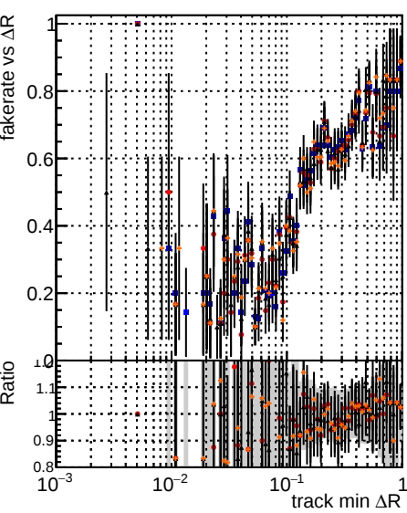
Fake rate vs \Delta R(\text{track, jet}) Duplicates Rate vs \Delta R(\text{track, jet}) Pileup rate vs \Delta R(\text{track, jet}) DOM mktFit Toriginal NEWHSMS95 ALLITERS-106
