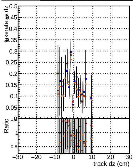
Fake rate vs dz Legend: DSM mkFit TOriginal_106 DSM mkFit TNEWHSMS95 DSM mkFit TALLITERS106
