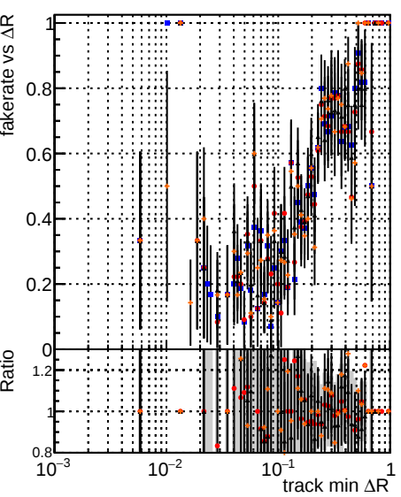
Fake rate vs \Delta R (track, jet) for DOM, mkFit, Original, NEWSM95, ALLTERS-106, and NEWSM95 ALLTERS-106 datasets.
