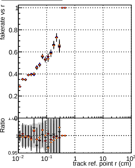
Fake rate vs v DOM mkFit Toriginal-106 DOM mkFit TNEW-106 DOM mkFit TNEW-SMS95 ALLITERS-106
