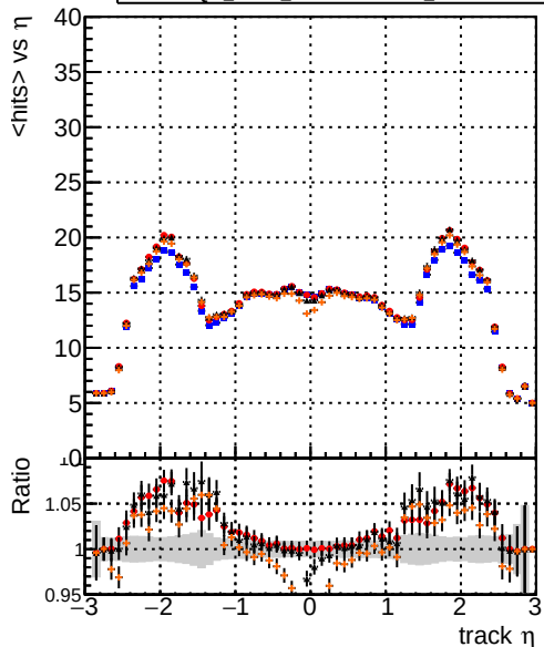
Legend: DQM_mkFit_TToriginal (blue line), DQM_mkFit_TToriginal-106 (red line with error bars), DQM_mkFit_TTNEWHSMS95_ALLITERS-106 (black line with error bars), DQM_mkFit_TTNEWHSMS90_ALLITERS-106 (orange line with error bars) mean hit
