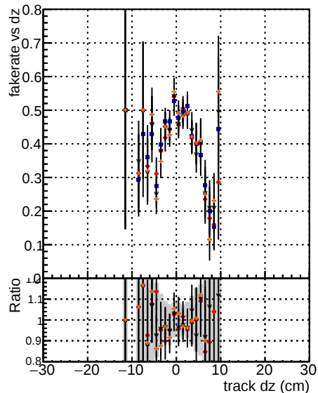
Fake rate vs dz Legend: BQM mktFit T-Original T-NEW T-ALLITERS
