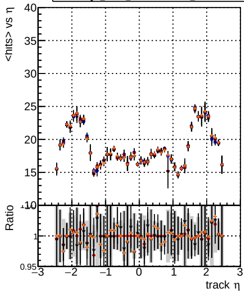
mean hit Legend: - DQM_mkFit_TToriginal (blue line with circles) - DQM_mkFit_TToriginal-106 (red line with circles) - DQM_mkFit_TTNEWHSMS95_ALLITERS-106 (black line with circles) - DQM_mkFit_TTNEWHSMS90_ALLITERS-106 (orange line with circles)
