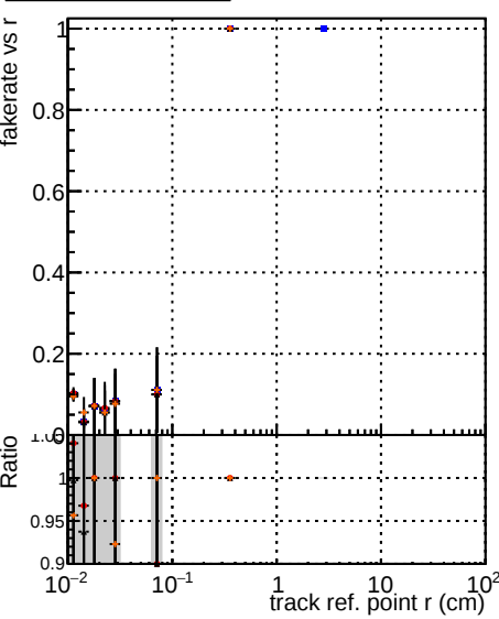
Fake rate vs v DOM mktFit Toriginal DOM mktFit TNEW S95 ALLITERS-106
